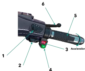
RIGHT - SIDE HANDLE CONTROLS
